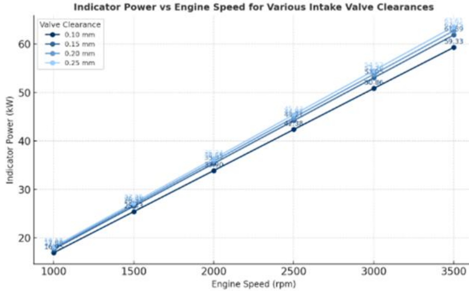
Figure 4. Indicator Power vs Engine speed
